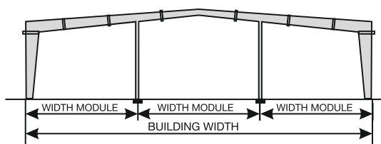
Multi-Span "2" (MS-2)
