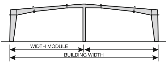
Multi-Span "1" (MS-1)
